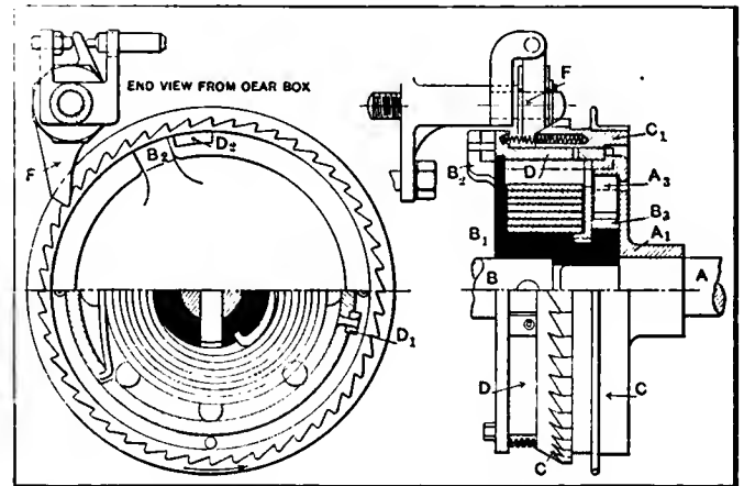
Fig. 3—Sectional view of Goodhart engine starter, an English invention
